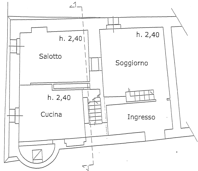
PIANO TERRENO
